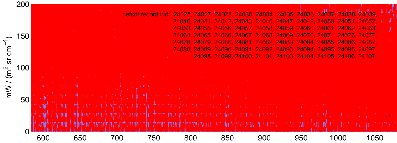
sh130507, REAL(LW) Radiances included in shis_130507_sci_lw.nc BLUE = OK (meaned by seg); RED = significant imaginary content
