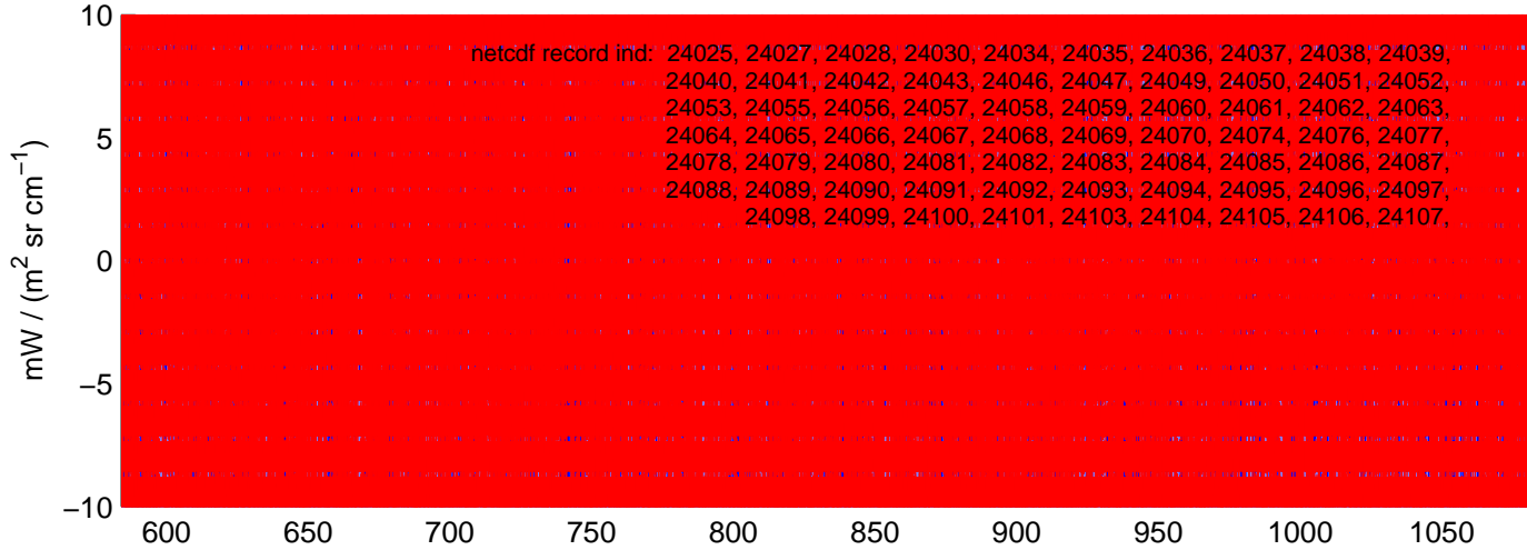
sh130507, Questionable (IMAG) LW Radiances included in shis_130507_sci_lw.nc BLUE = OK (meaned by seg); RED = significant imaginary content
