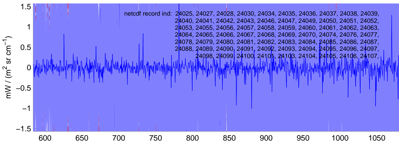
sh130507, PHASE(LW) Radiances included in shis_130507_sci_lw.nc BLUE = OK (meaned by seg); RED = significant imaginary content
