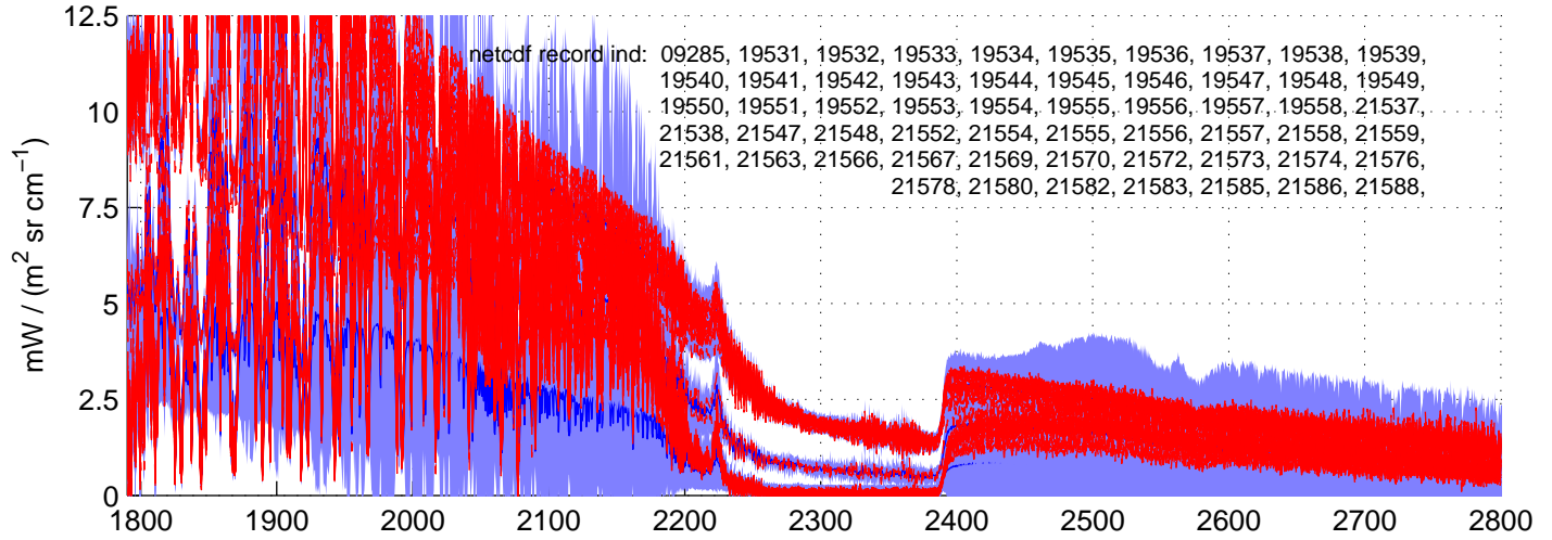
sh130503, REAL(SW) Radiances included in shis_130503_sci_sw.nc BLUE = OK (meaned by seg); RED = significant imaginary content
