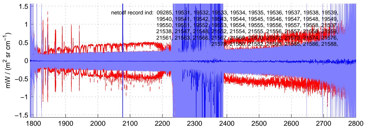
sh130503, PHASE(SW) Radiances included in shis_130503_sci_sw.nc BLUE = OK (meaned by seg); RED = significant imaginary content
