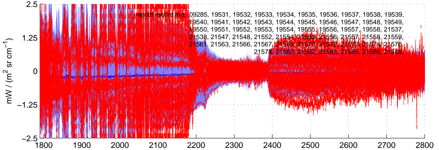
sh130503, IMAG(SW) Radiances included in shis_130503_sci_sw.nc BLUE = OK (meaned by seg); RED = significant imaginary content
