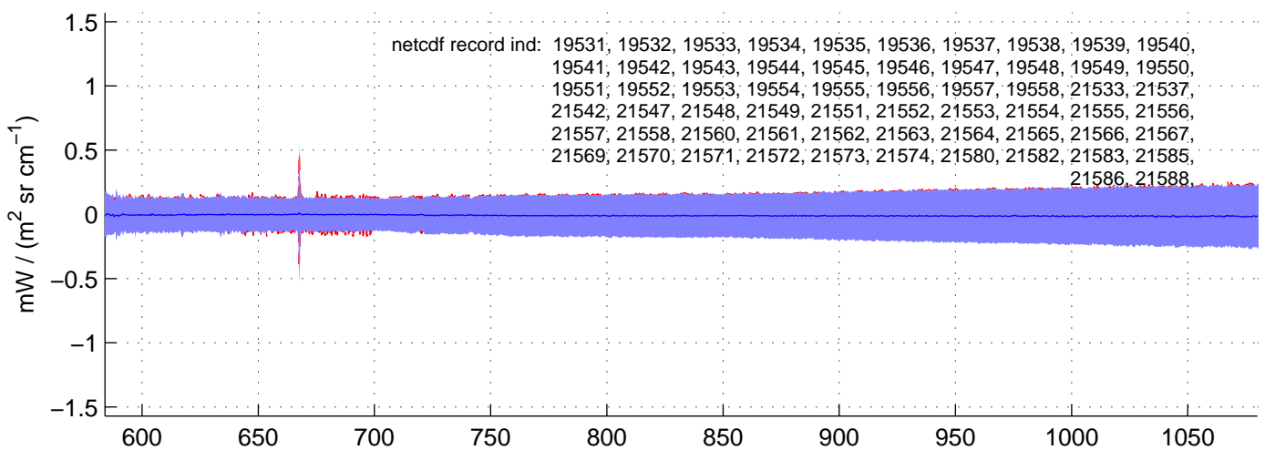
sh130503, PHASE(LW) Radiances included in shis_130503_sci_lw.nc BLUE = OK (meaned by seg); RED = significant imaginary content
