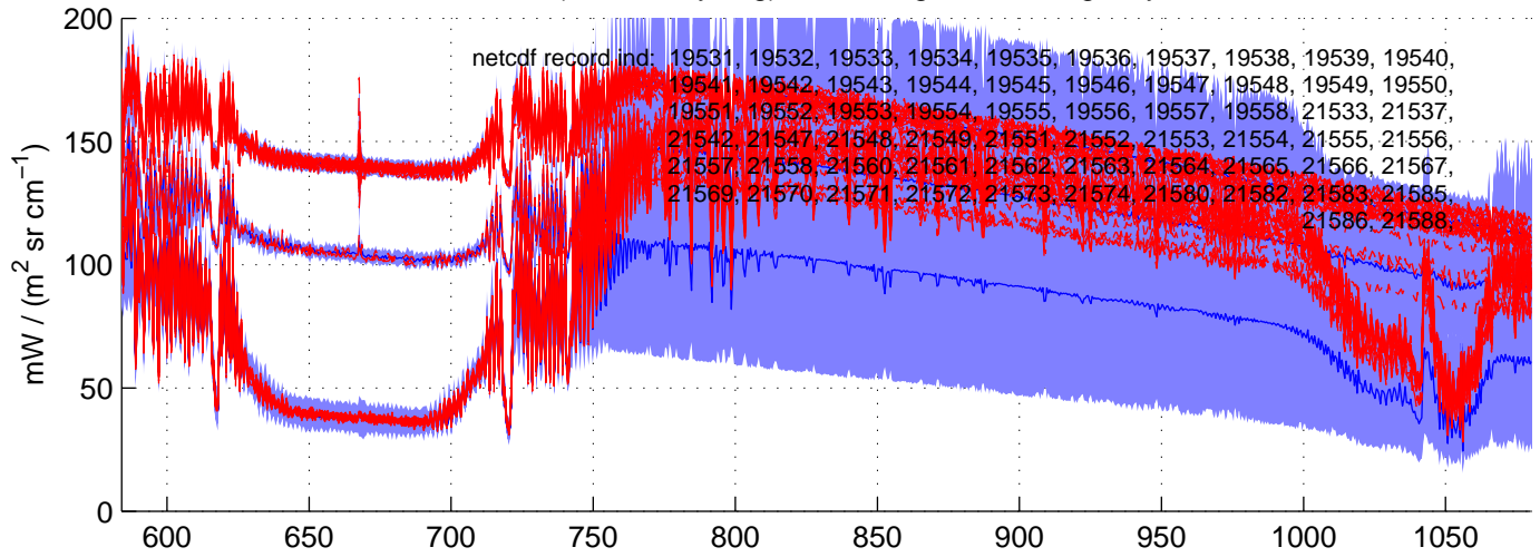
sh130503, REAL(LW) Radiances included in shis_130503_sci_lw.nc BLUE = OK (meaned by seg); RED = significant imaginary content
