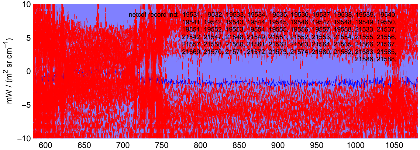
sh130503, Questionable (IMAG) LW Radiances included in shis_130503_sci_lw.nc BLUE = OK (meaned by seg); RED = significant imaginary content
