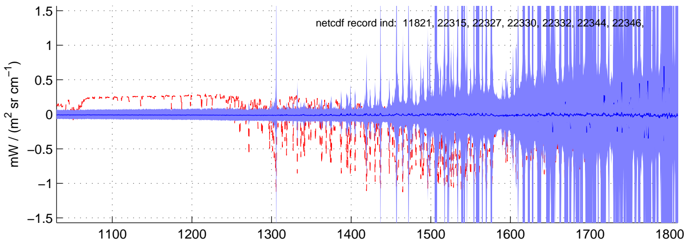
sh130502, PHASE(MW) Radiances included in shis_130502_sci_mw.nc BLUE = OK (meaned by seg); RED = significant imaginary content
