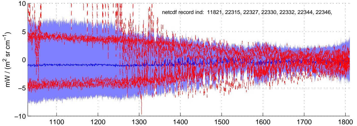
sh130502, IMAG(MW) Radiances included in shis_130502_sci_mw.nc BLUE = OK (meaned by seg); RED = significant imaginary content
