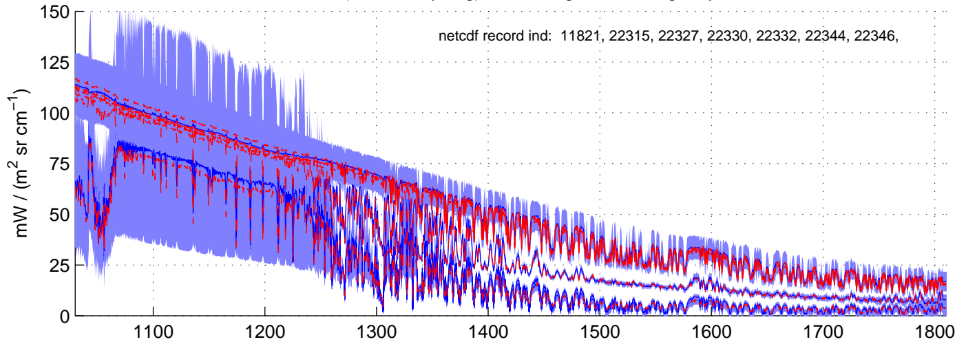
sh130502, REAL(MW) Radiances included in shis_130502_sci_mw.nc BLUE = OK (meaned by seg); RED = significant imaginary content
