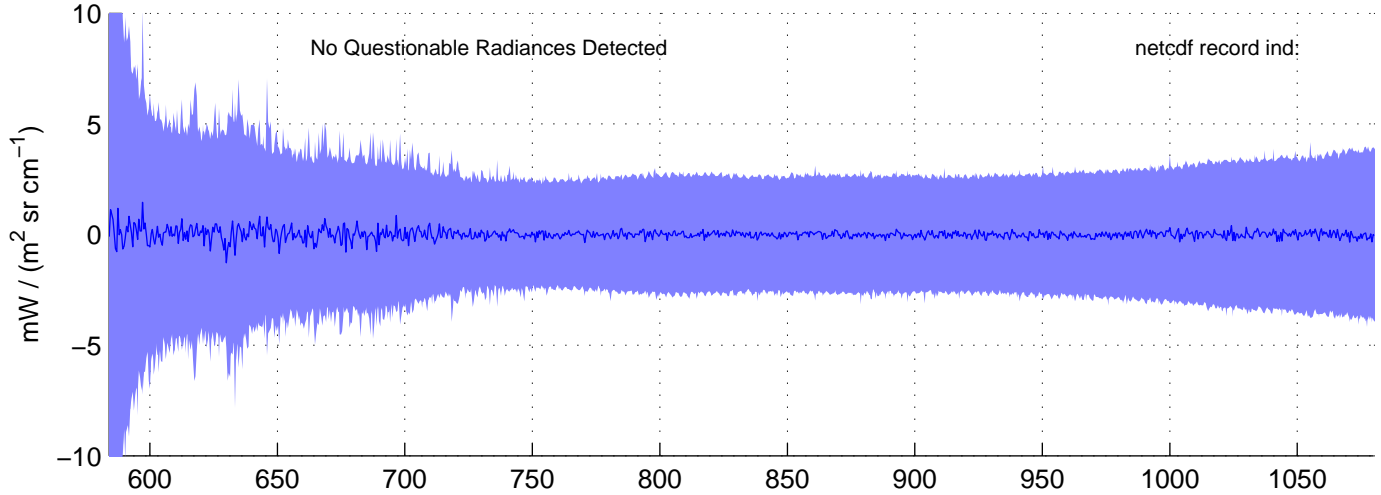
sh121006, Questionable (IMAG) LW Radiances included in shis_121006_sci_lw.nc BLUE = OK (meaned by seg); RED = significant imaginary content
