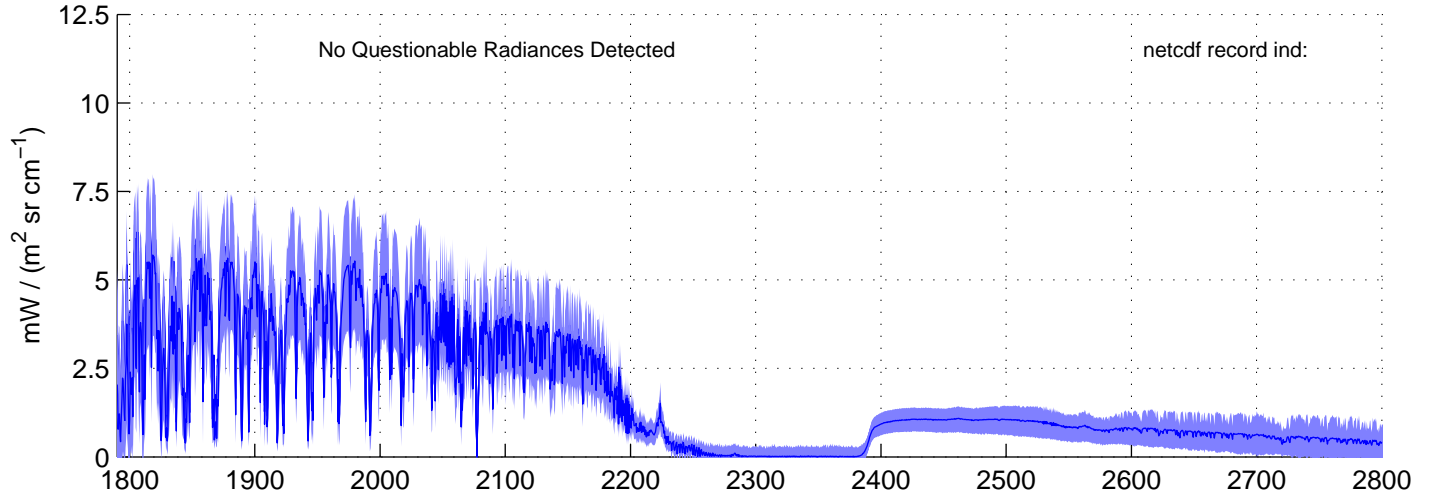
sh121006, REAL(SW) Radiances included in shis_121006_sci_sw.nc BLUE = OK (meaned by seg); RED = significant imaginary content
