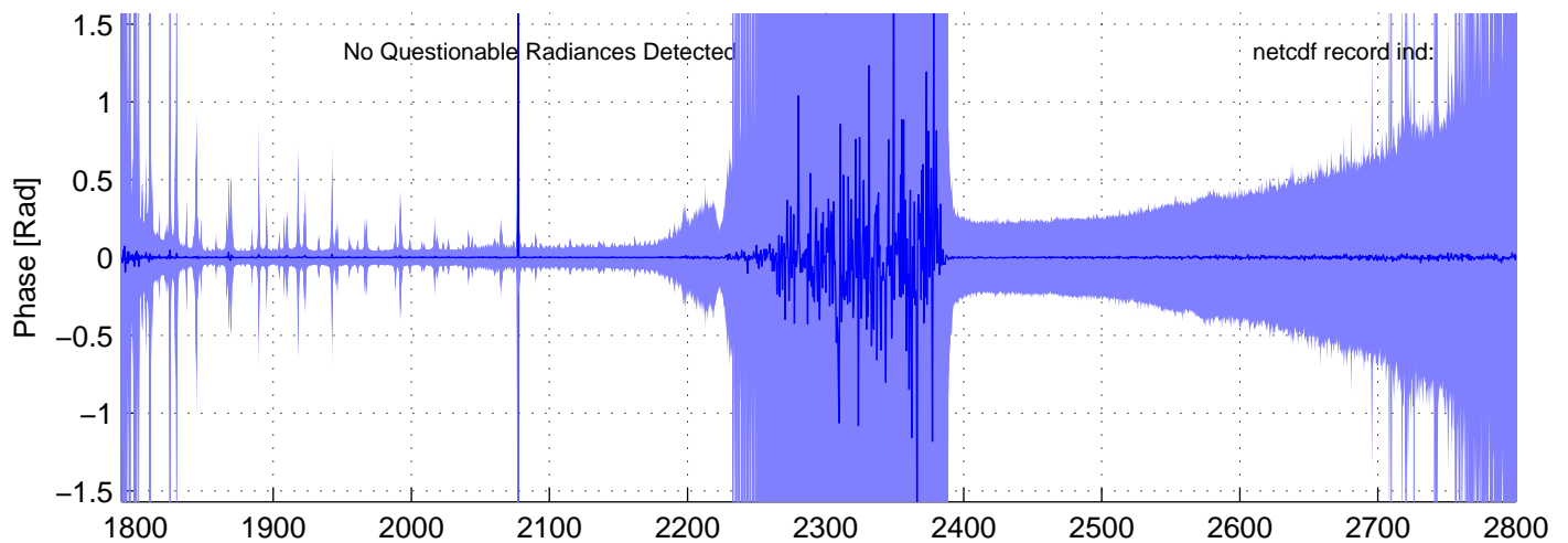
sh121006, PHASE(SW) Radiances included in shis_121006_sci_sw.nc BLUE = OK (meaned by seg); RED = significant imaginary content
