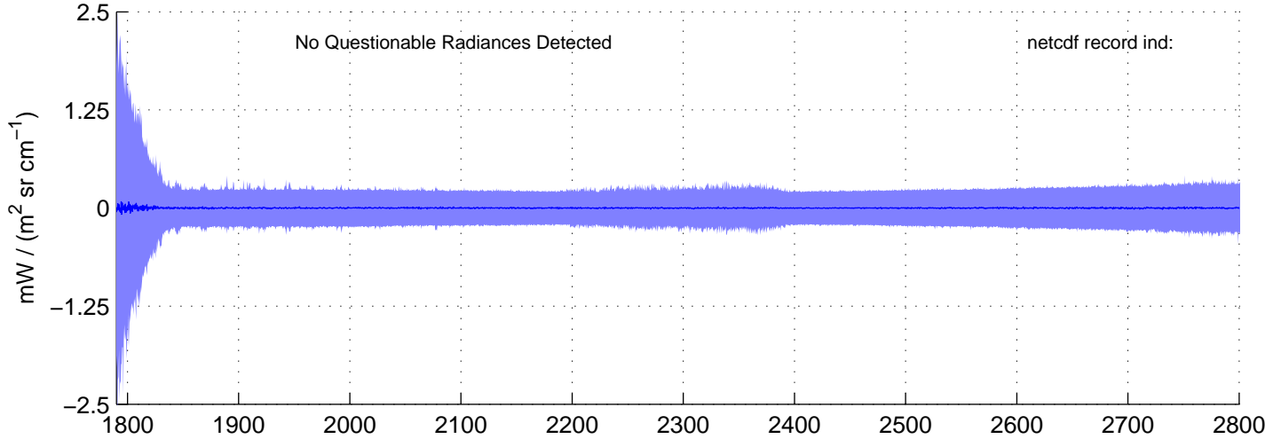
sh121006, IMAG(SW) Radiances included in shis_121006_sci_sw.nc BLUE = OK (meaned by seg); RED = significant imaginary content
