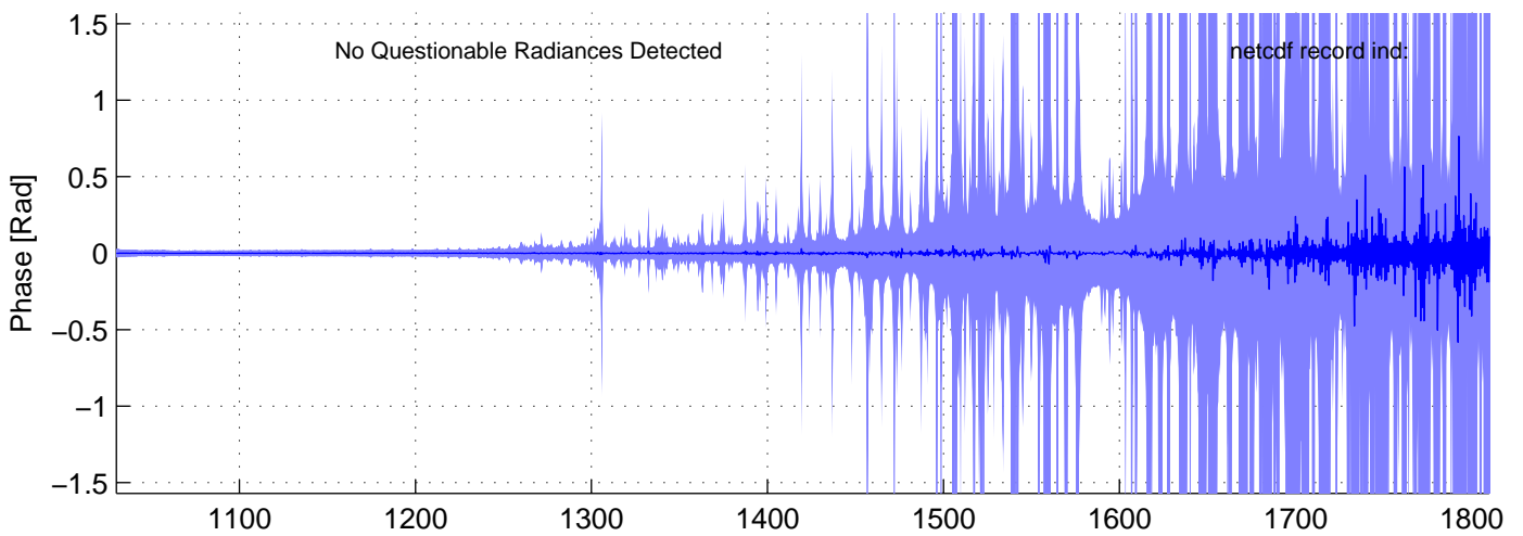
sh121006, PHASE(MW) Radiances included in shis_121006_sci_mw.nc BLUE = OK (meaned by seg); RED = significant imaginary content
