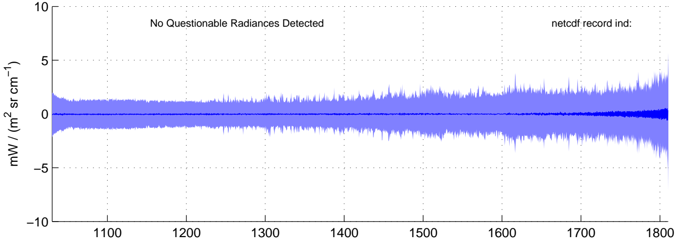
sh121006, IMAG(MW) Radiances included in shis_121006_sci_mw.nc BLUE = OK (meaned by seg); RED = significant imaginary content
