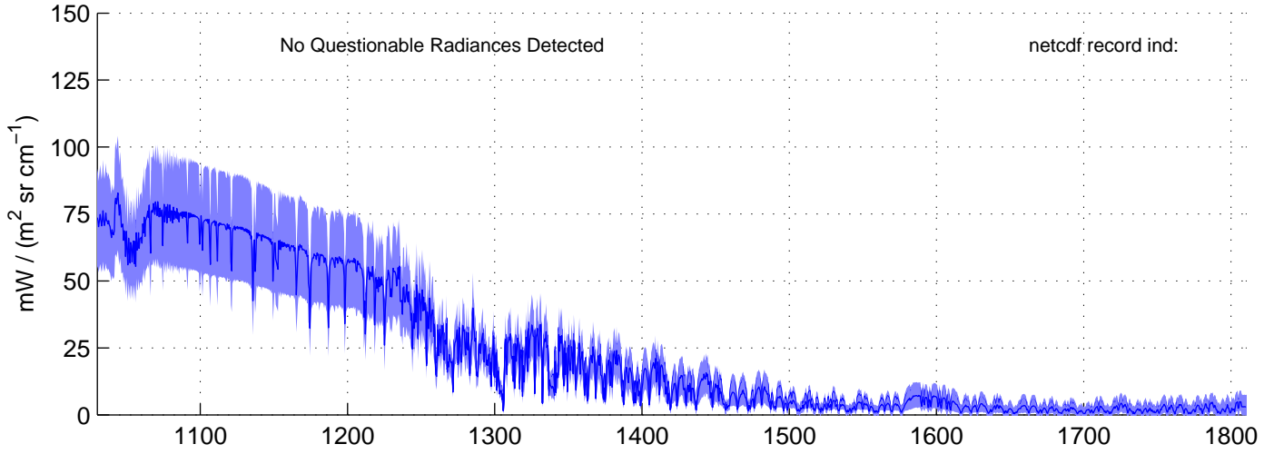
sh121006, REAL(MW) Radiances included in shis_121006_sci_mw.nc BLUE = OK (meaned by seg); RED = significant imaginary content
