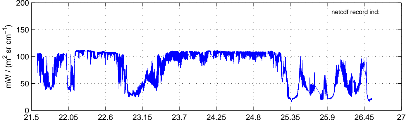
sh120926 Mean Radiance 895.00 – 900.00, good segments
