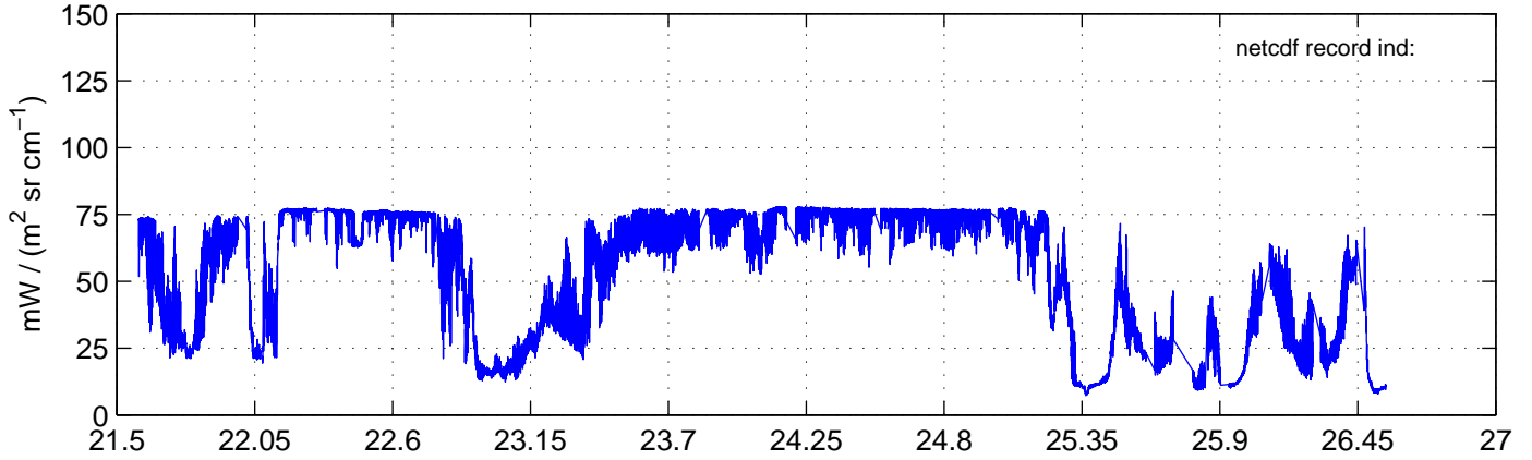
sh120926 Mean Radiance 1093.00 – 1097.00, good segments
