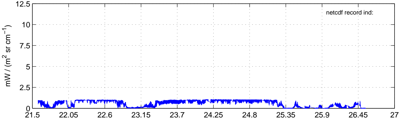
sh120926 Mean Radiance 2500.00 – 2510.00, good segments
