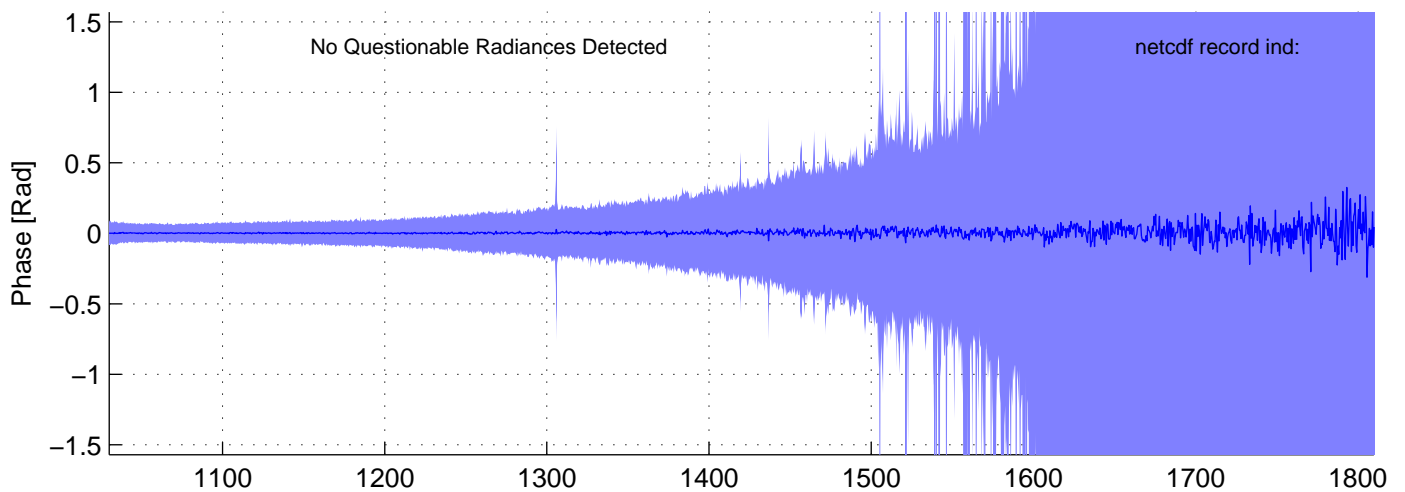
sh120926, PHASE(MW) Radiances included in shis_120926_sci_mw.nc BLUE = OK (meaned by seg); RED = significant imaginary content
