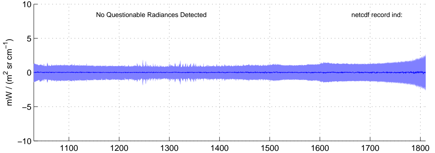
sh120926, IMAG(MW) Radiances included in shis_120926_sci_mw.nc BLUE = OK (meaned by seg); RED = significant imaginary content
