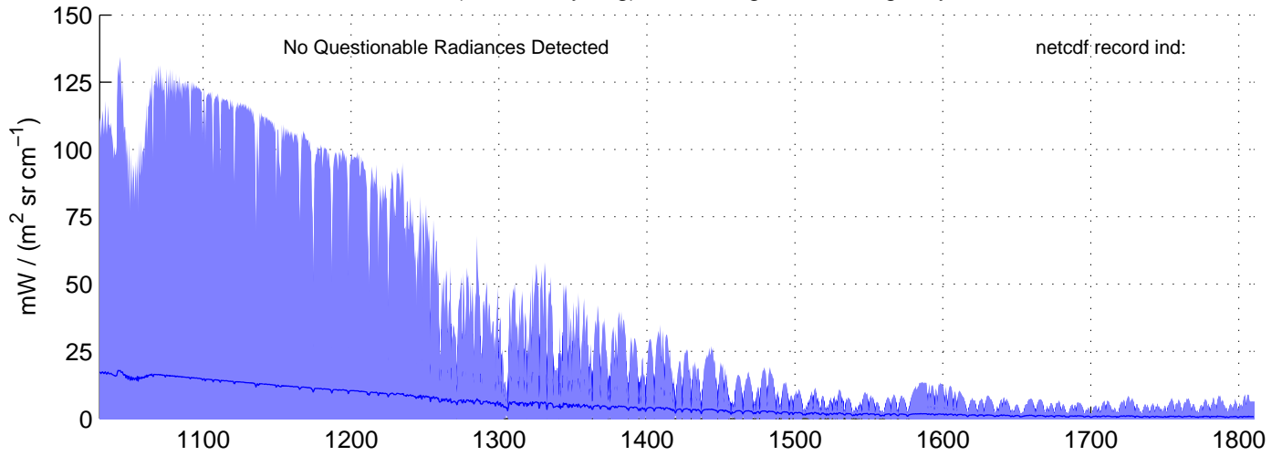
sh120926, REAL(MW) Radiances included in shis_120926_sci_mw.nc BLUE = OK (meaned by seg); RED = significant imaginary content
