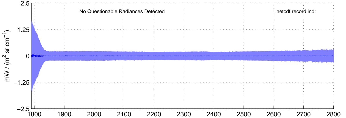
sh120926, IMAG(SW) Radiances included in shis_120926_sci_sw.nc BLUE = OK (meaned by seg); RED = significant imaginary content
