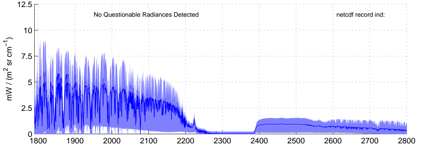
sh120926, REAL(SW) Radiances included in shis_120926_sci_sw.nc BLUE = OK (meaned by seg); RED = significant imaginary content
