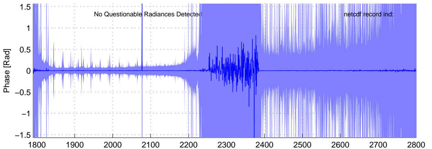
sh120926, PHASE(SW) Radiances included in shis_120926_sci_sw.nc BLUE = OK (meaned by seg); RED = significant imaginary content
