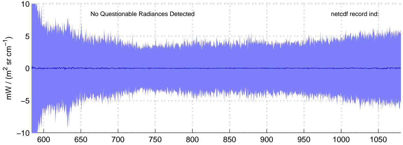
sh120926, Questionable (IMAG) LW Radiances included in shis_120926_sci_lw.nc BLUE = OK (meaned by seg); RED = significant imaginary content
