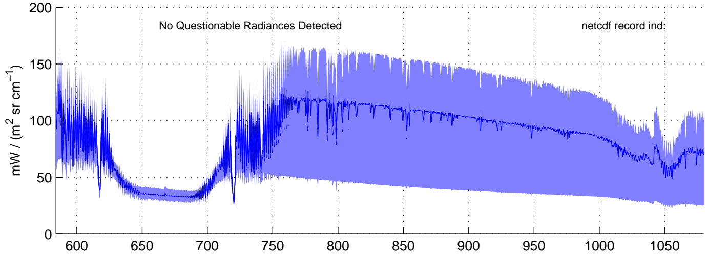
sh120926, REAL(LW) Radiances included in shis_120926_sci_lw.nc BLUE = OK (meaned by seg); RED = significant imaginary content
