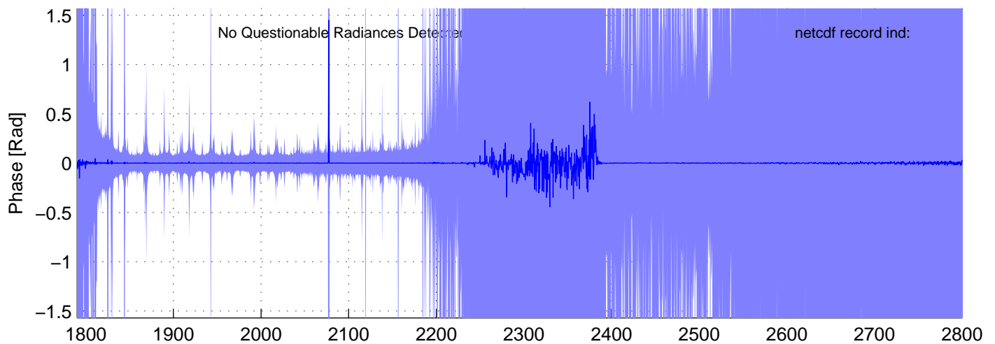
sh120922, PHASE(SW) Radiances included in shis_120922_sci_sw.nc BLUE = OK (meaned by seg); RED = significant imaginary content
