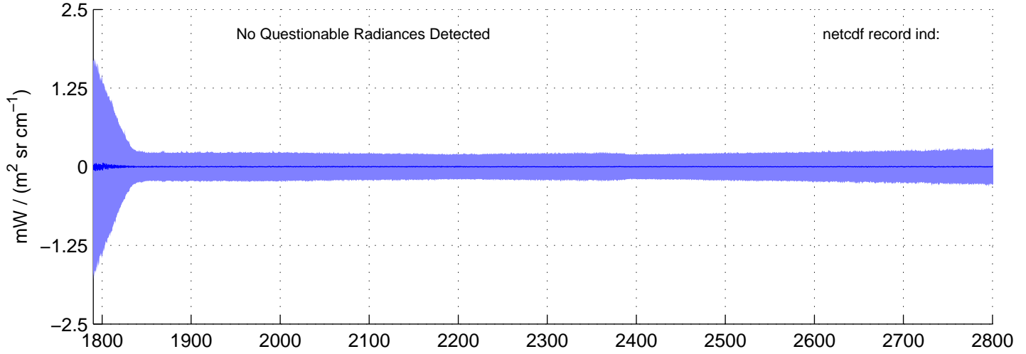
sh120922, IMAG(SW) Radiances included in shis_120922_sci_sw.nc BLUE = OK (meaned by seg); RED = significant imaginary content
