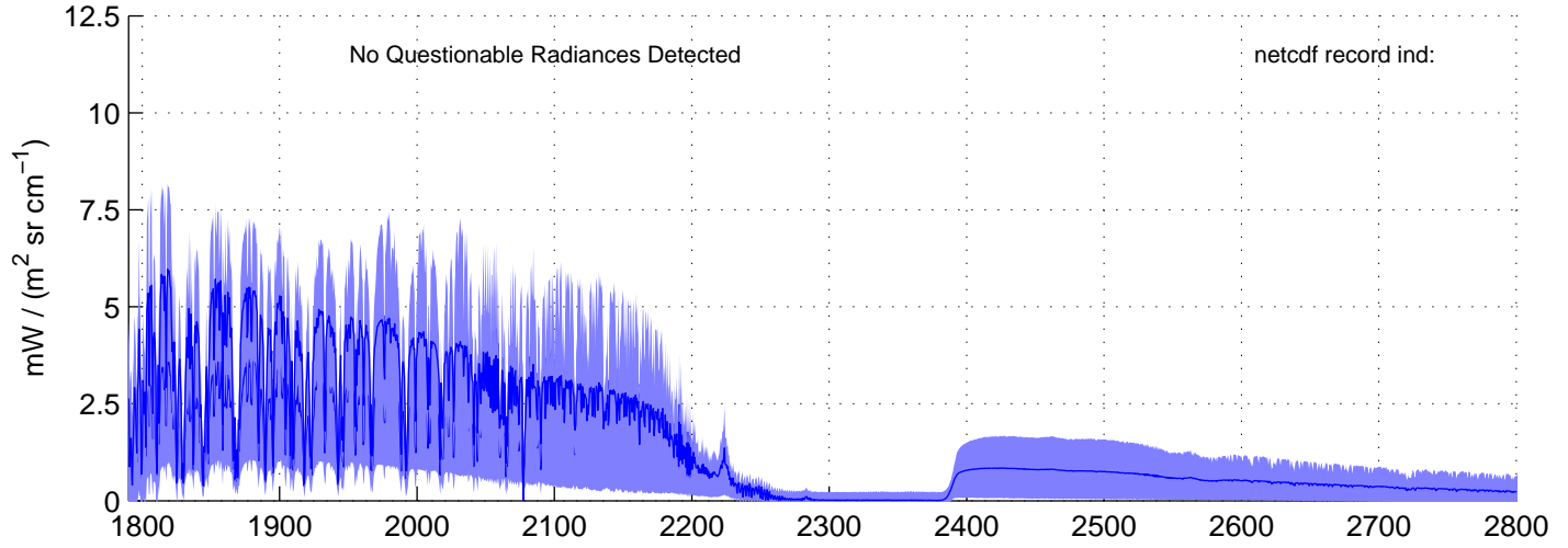
sh120922, REAL(SW) Radiances included in shis_120922_sci_sw.nc BLUE = OK (meaned by seg); RED = significant imaginary content
