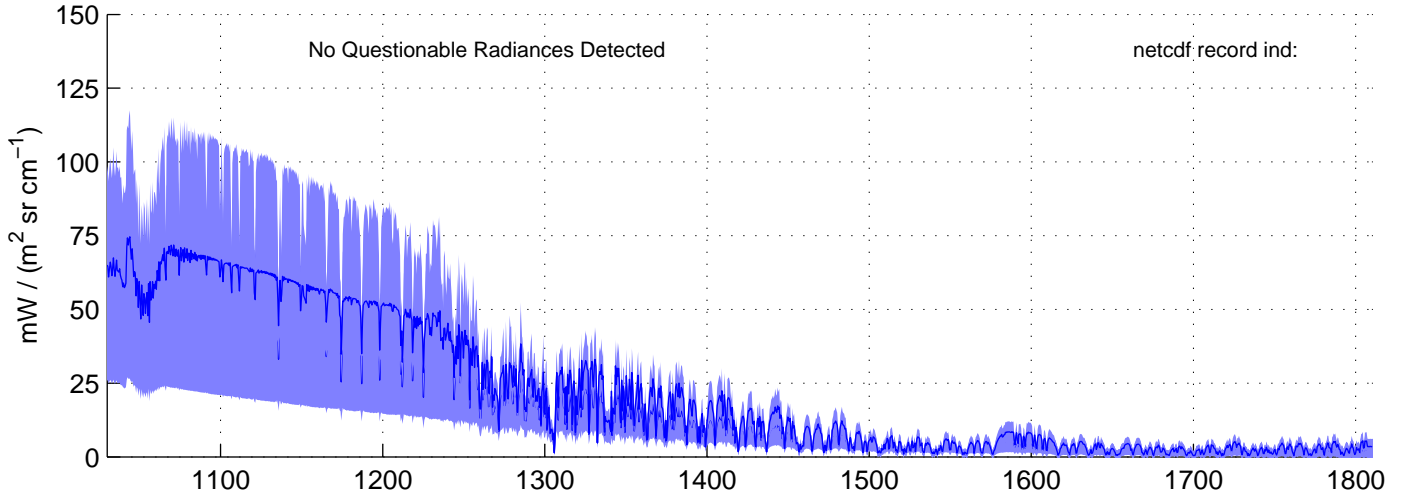
sh120922, REAL(MW) Radiances included in shis_120922_sci_mw.nc BLUE = OK (meaned by seg); RED = significant imaginary content
