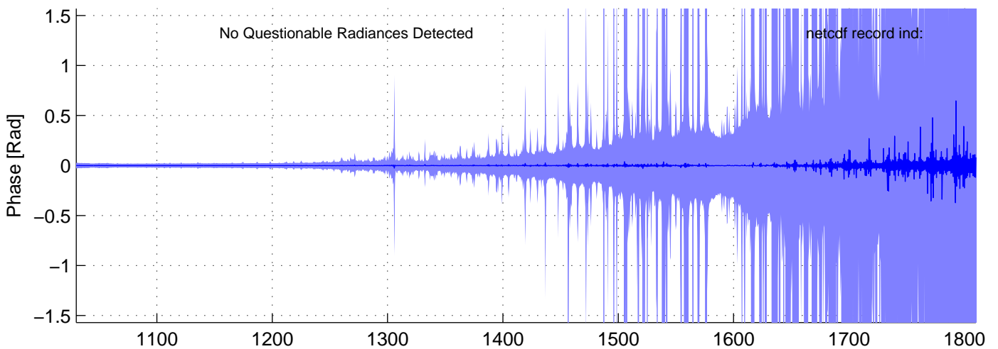
sh120922, PHASE(MW) Radiances included in shis_120922_sci_mw.nc BLUE = OK (meaned by seg); RED = significant imaginary content
