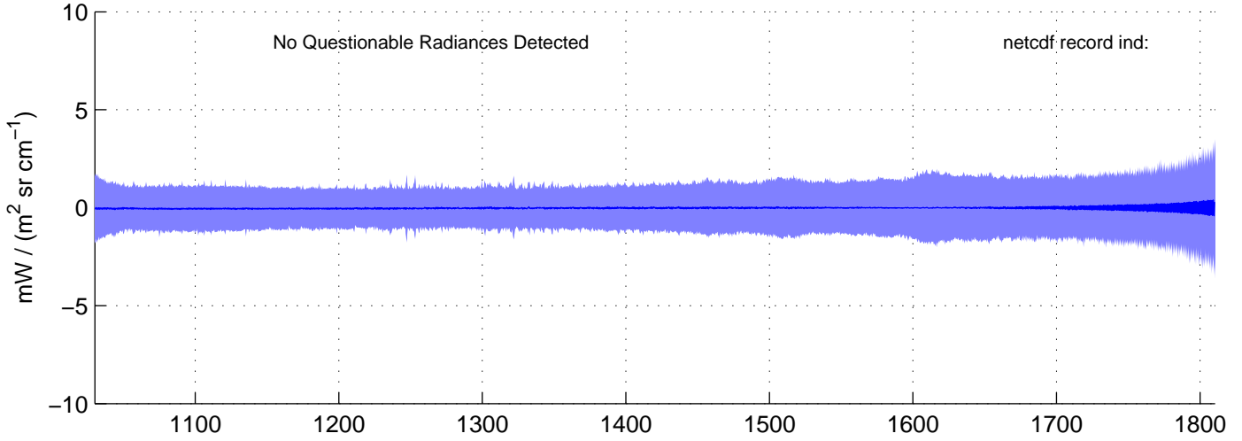
sh120922, IMAG(MW) Radiances included in shis_120922_sci_mw.nc BLUE = OK (meaned by seg); RED = significant imaginary content
