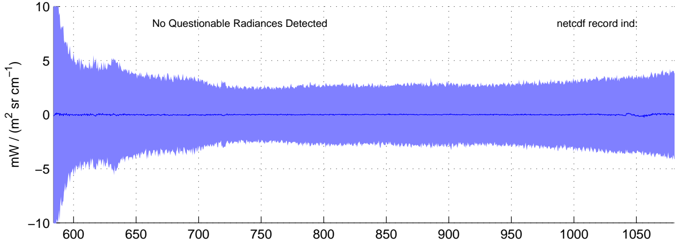
sh120922, Questionable (IMAG) LW Radiances included in shis_120922_sci_lw.nc BLUE = OK (meaned by seg); RED = significant imaginary content
