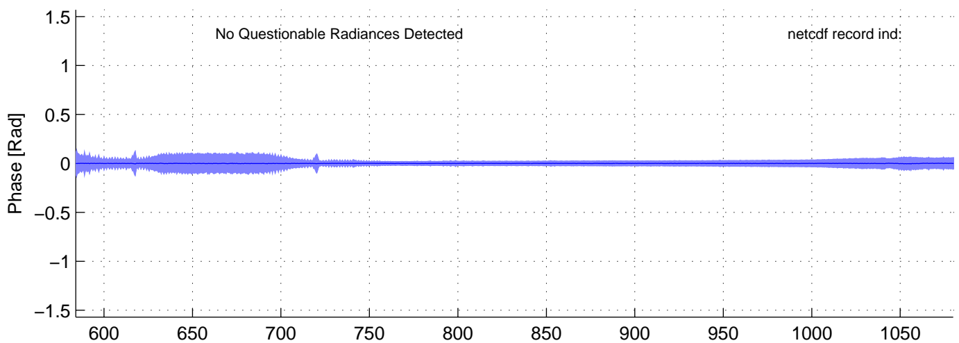
sh120922, PHASE(LW) Radiances included in shis_120922_sci_lw.nc BLUE = OK (meaned by seg); RED = significant imaginary content
