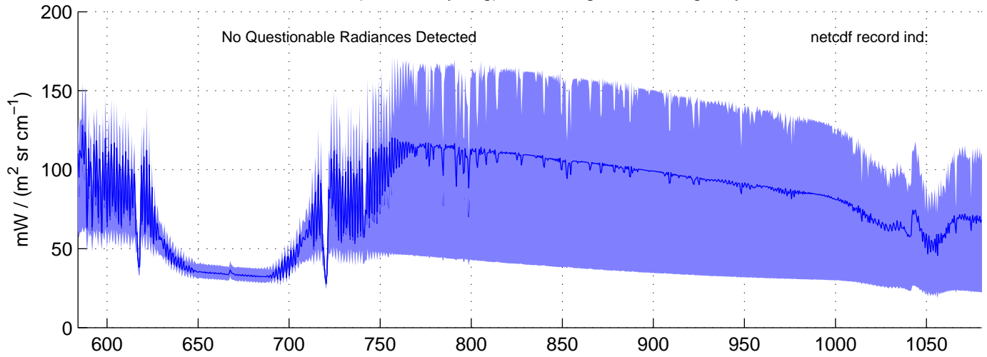
sh120922, REAL(LW) Radiances included in shis_120922_sci_lw.nc BLUE = OK (meaned by seg); RED = significant imaginary content
