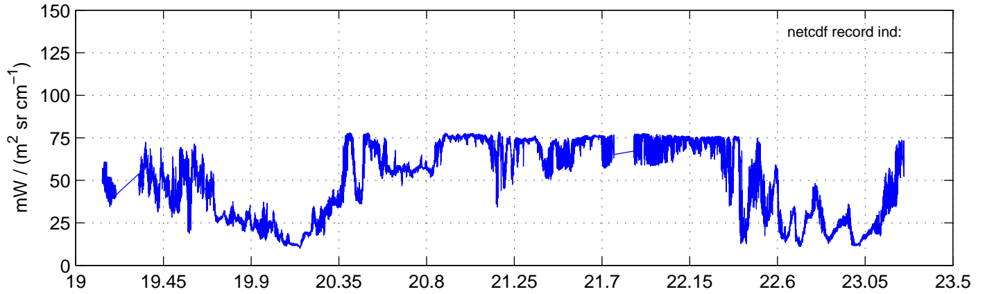
sh120919 Mean Radiance 1093.00 – 1097.00, good segments
