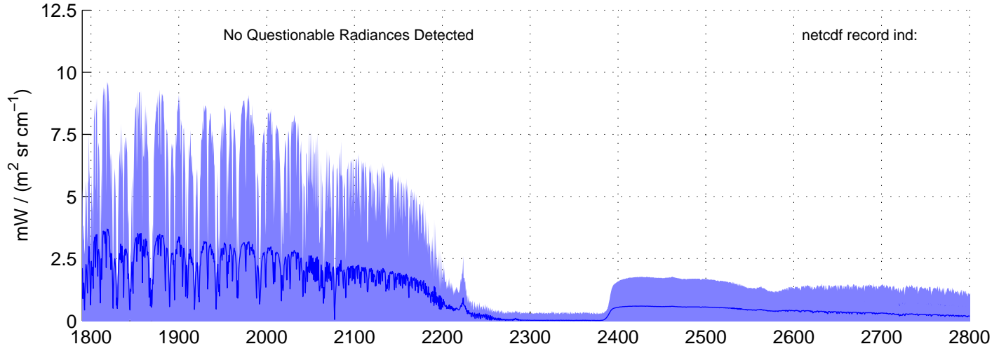
sh120919, REAL(SW) Radiances included in shis_120919_sci_sw.nc BLUE = OK (meaned by seg); RED = significant imaginary content
