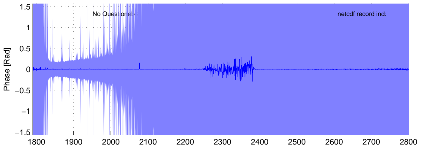
sh120919, PHASE(SW) Radiances included in shis_120919_sci_sw.nc BLUE = OK (meaned by seg); RED = significant imaginary content
