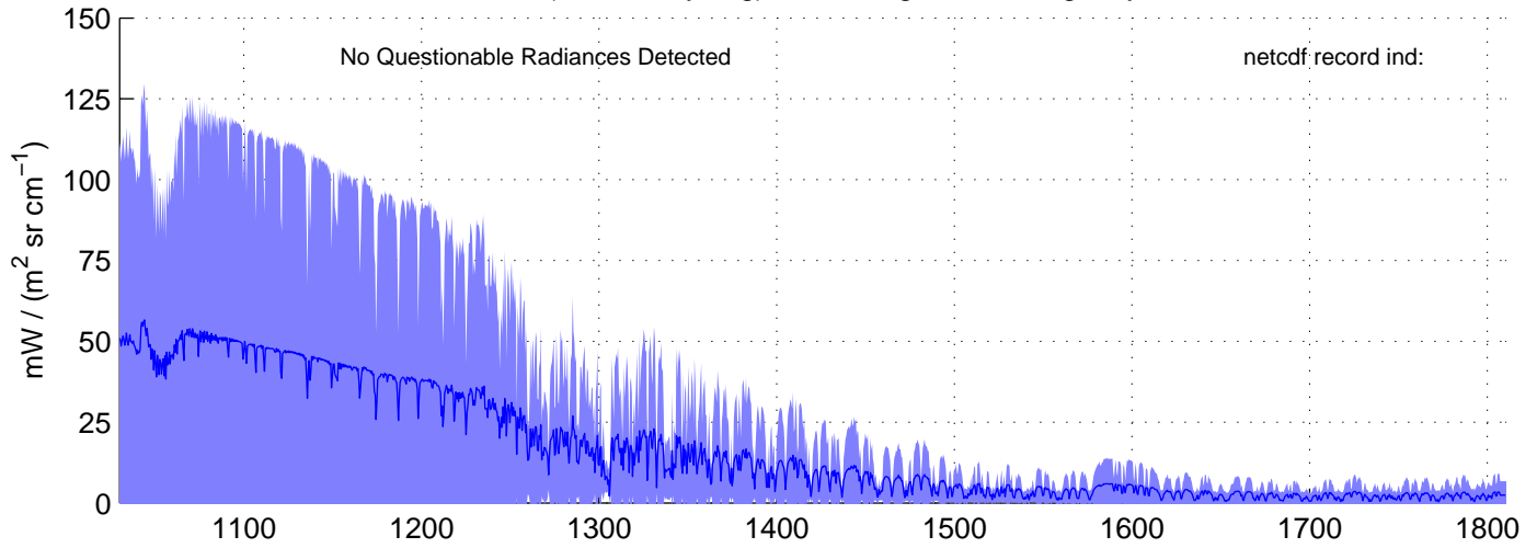
sh120919, REAL(MW) Radiances included in shis_120919_sci_mw.nc BLUE = OK (meaned by seg); RED = significant imaginary content
