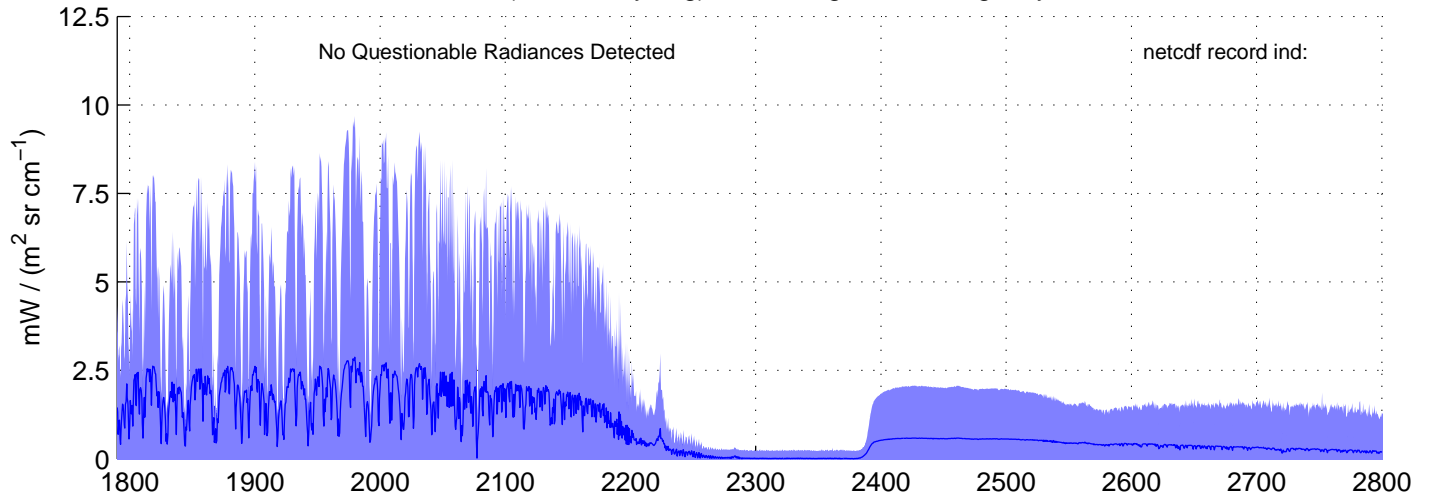
sh120914, REAL(SW) Radiances included in shis_120914_sci_sw.nc BLUE = OK (meaned by seg); RED = significant imaginary content
