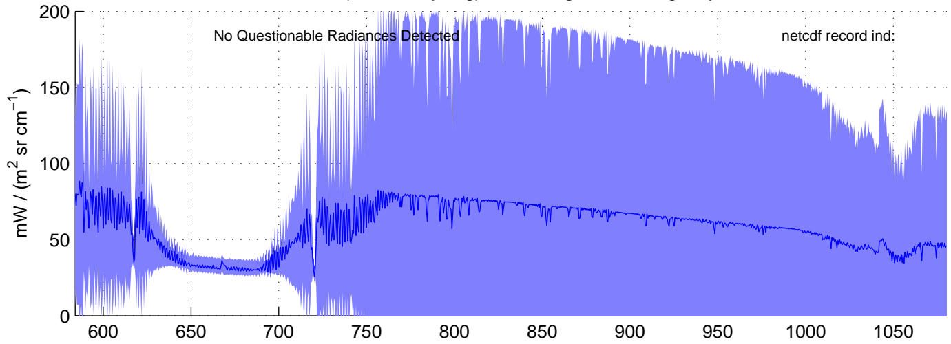
sh120914, REAL(LW) Radiances included in shis_120914_sci_lw.nc BLUE = OK (meaned by seg); RED = significant imaginary content
