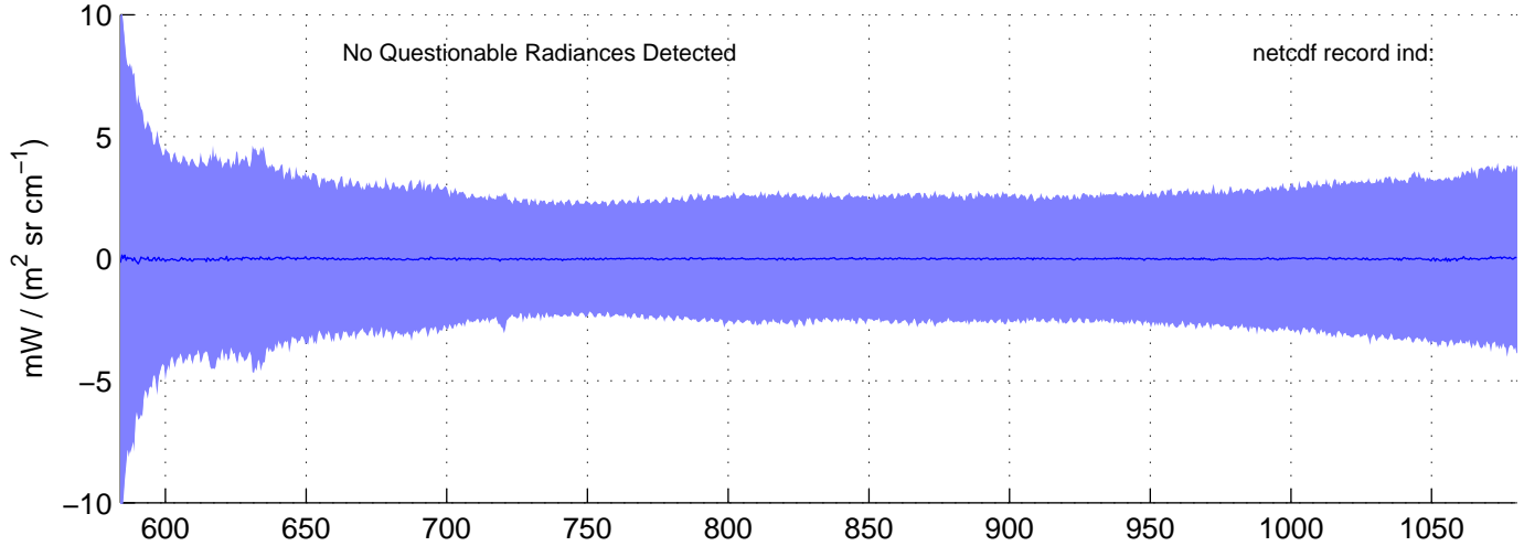
sh120911, Questionable (IMAG) LW Radiances included in shis_120911_sci_lw.nc BLUE = OK (meaned by seg); RED = significant imaginary content
