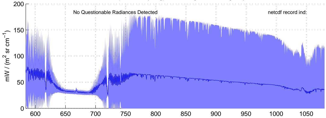
sh120911, REAL(LW) Radiances included in shis_120911_sci_lw.nc BLUE = OK (meaned by seg); RED = significant imaginary content
