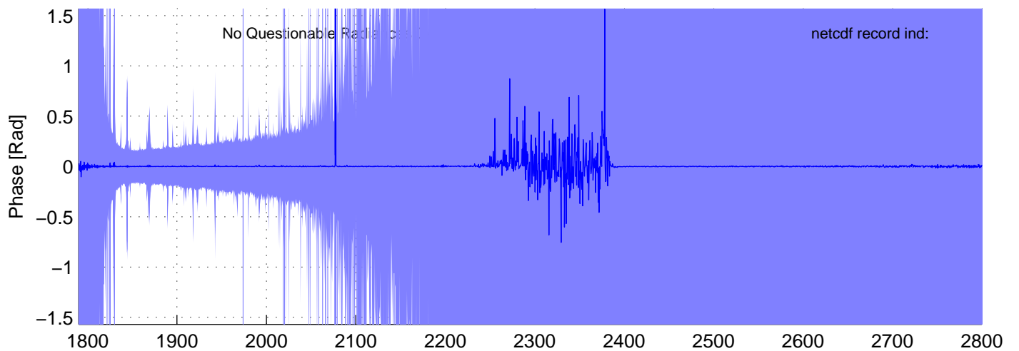
sh120911, PHASE(SW) Radiances included in shis_120911_sci_sw.nc BLUE = OK (meaned by seg); RED = significant imaginary content
