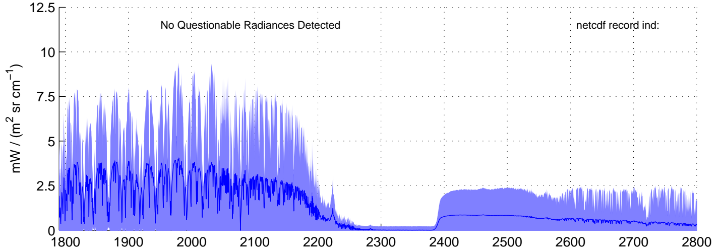
sh120911, REAL(SW) Radiances included in shis_120911_sci_sw.nc BLUE = OK (meaned by seg); RED = significant imaginary content
