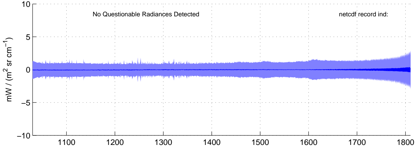
sh120911, IMAG(MW) Radiances included in shis_120911_sci_mw.nc BLUE = OK (meaned by seg); RED = significant imaginary content
