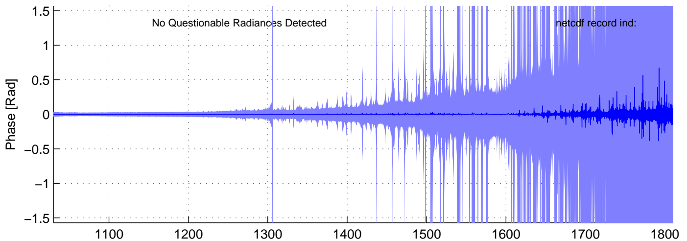
sh120911, PHASE(MW) Radiances included in shis_120911_sci_mw.nc BLUE = OK (meaned by seg); RED = significant imaginary content
