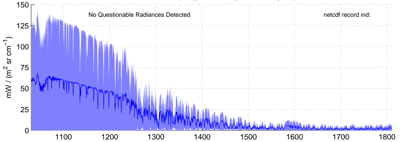
sh120911, REAL(MW) Radiances included in shis_120911_sci_mw.nc BLUE = OK (meaned by seg); RED = significant imaginary content
