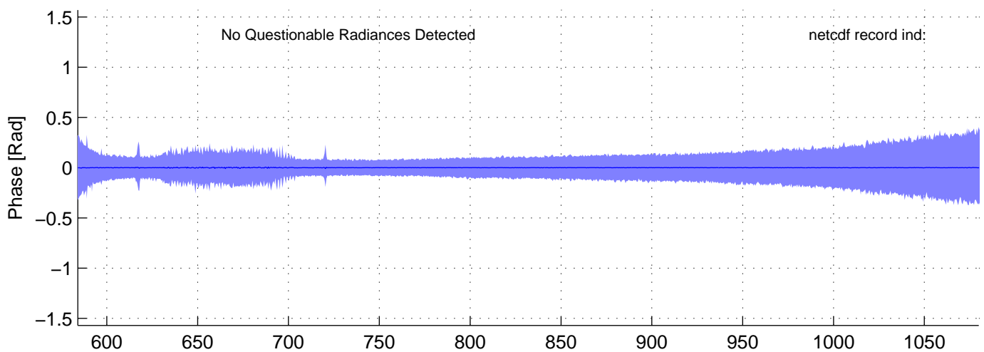
sh120906, PHASE(LW) Radiances included in shis_120906_sci_lw.nc BLUE = OK (meaned by seg); RED = significant imaginary content
