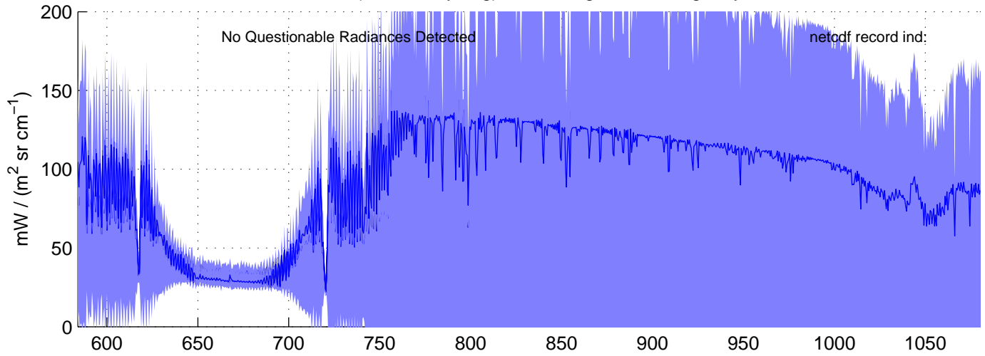
sh120906, REAL(LW) Radiances included in shis_120906_sci_lw.nc BLUE = OK (meaned by seg); RED = significant imaginary content
