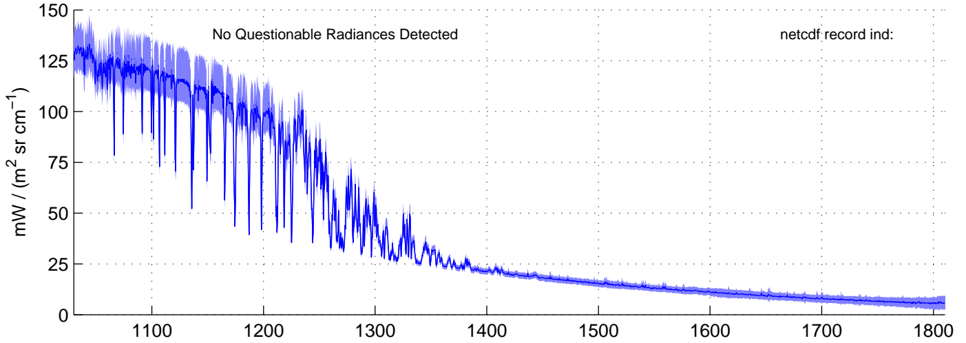
sh120828, REAL(MW) Radiances included in shis_120828_sci_mw.nc BLUE = OK (meaned by seg); RED = significant imaginary content
