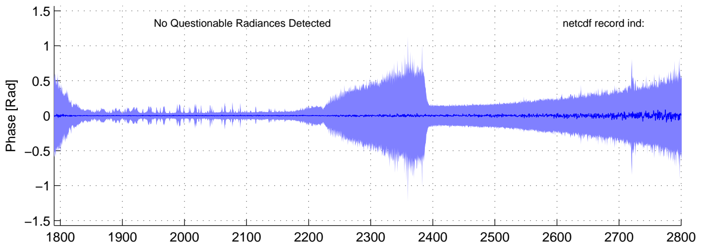
sh120828, PHASE(SW) Radiances included in shis_120828_sci_sw.nc BLUE = OK (meaned by seg); RED = significant imaginary content
