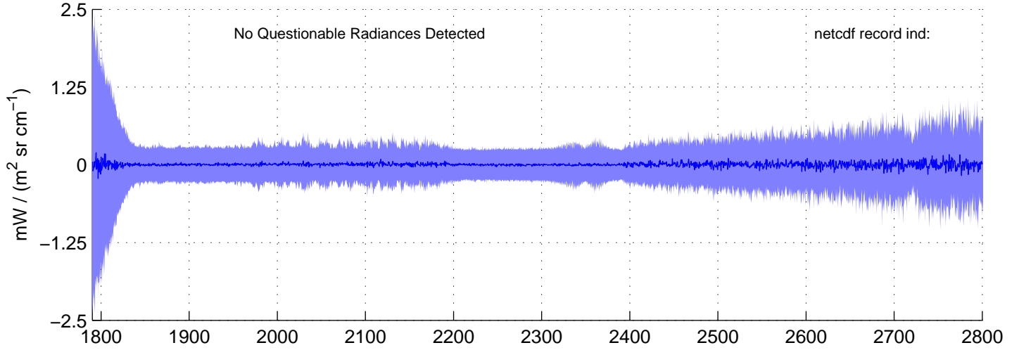
sh120828, IMAG(SW) Radiances included in shis_120828_sci_sw.nc BLUE = OK (meaned by seg); RED = significant imaginary content
