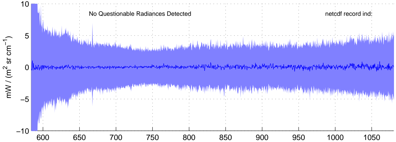
sh120828, Questionable (IMAG) LW Radiances included in shis_120828_sci_lw.nc BLUE = OK (meaned by seg); RED = significant imaginary content
